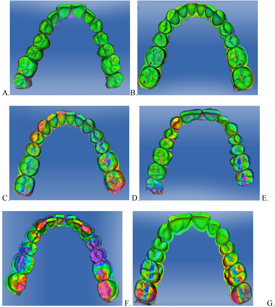
Fig. 3 Difference pattern between repeated impression (precision); color graded from -100\mu\text{m} (purple) to +100\mu\text{m} (red). A, VSE. B, VSES. C, VSES-D. D, POE. E, ALG. F, CER. G, OC. H, LAV. I, T-Def. K, ITE. L, TRI. M, TRC. .
