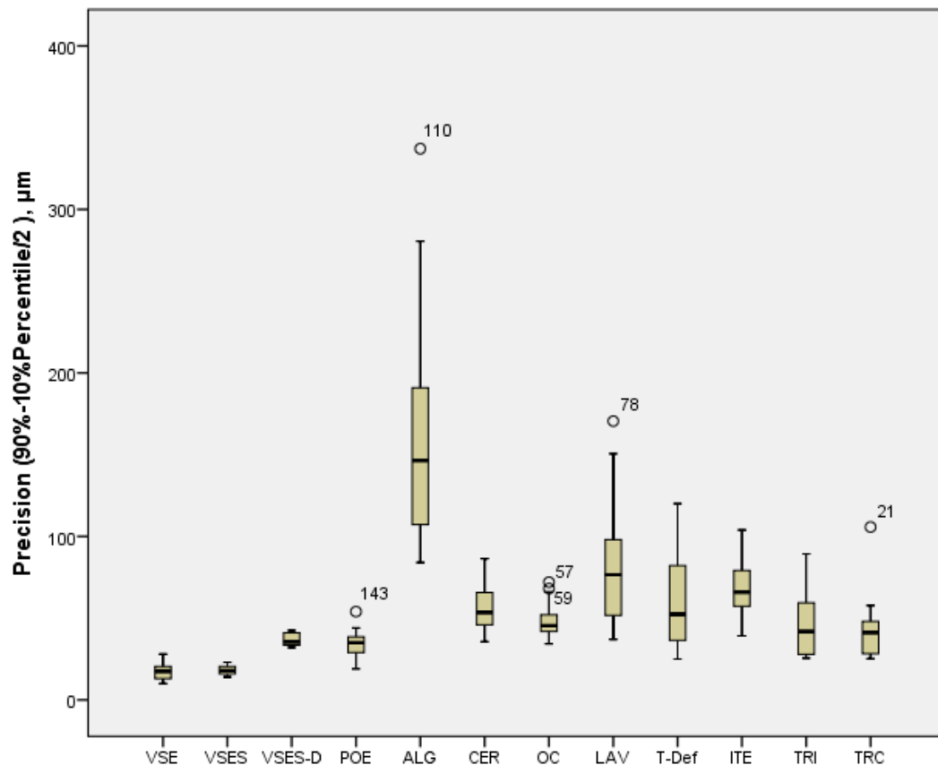
Fig. 2. Precision of conventional and digital complete arch impression in vivo ( \mu\text{m} ).
