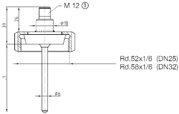
Dimensions (in mm) Connector 4-pin
