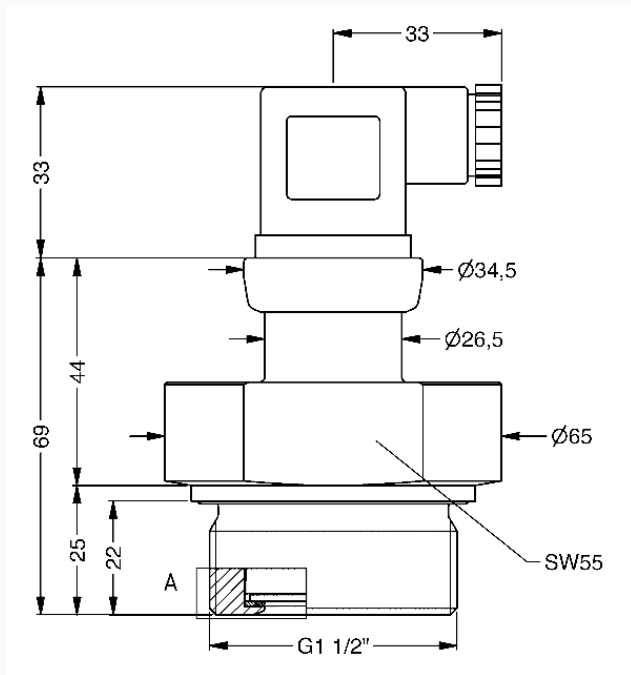
Dimensions (mm)
