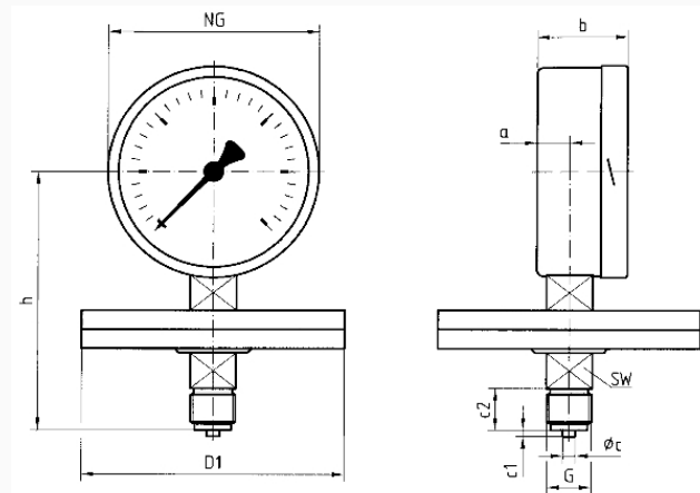
bottom connection, measuring flange \varnothing 160
