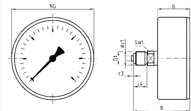
NG 80/100 – Anschluss axial
