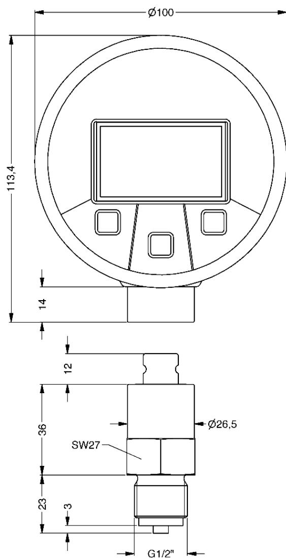
digital pressure gauge DIM 30
